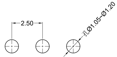
Recommended P.C.B Layout General Tolerance±0.05 T=1.60mm
